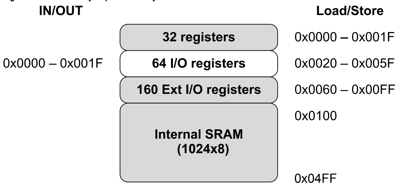
Figure 8-4. Data Memory Map with 1024 byte internal data SRAM
